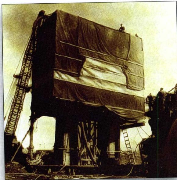
The "curing cabin" in-place at pier #7 ready for the final ("E") pour of concrete. A canvas pipe pumped concrete into the pier from the pump-crete mixer at the bottom right. Opposite page: The completed bridge which was dedicated 4 July, 1953.
