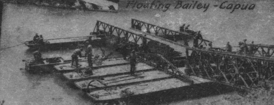
Floating Bailey - Capua
